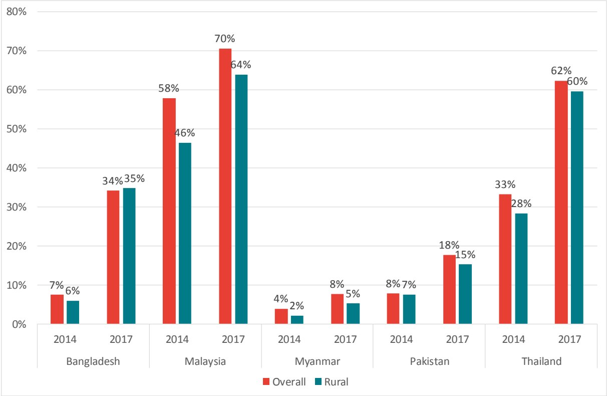
Figure 20: Percentage of population who made or received digital payments* in the past year
